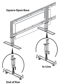
Connections Frame Leg — In-Line and End-of-Run Condition
